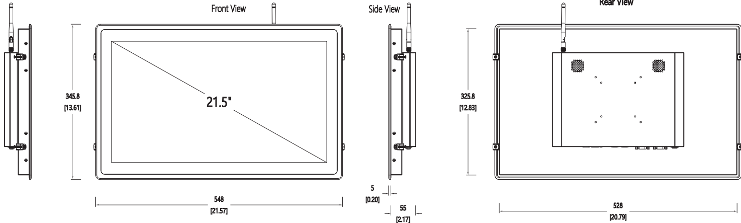
Rear View
